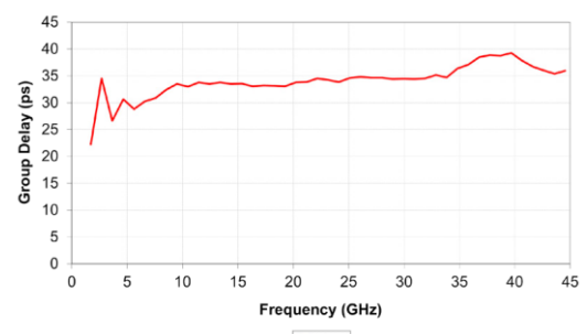
Group Delay
