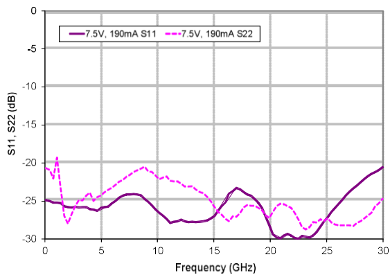
S11, S22
