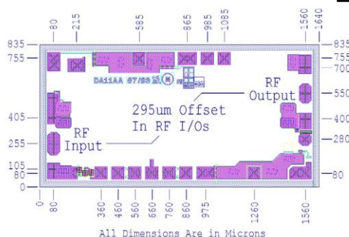
30GHz bonding diagram
