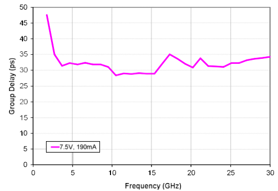
Group Delay
