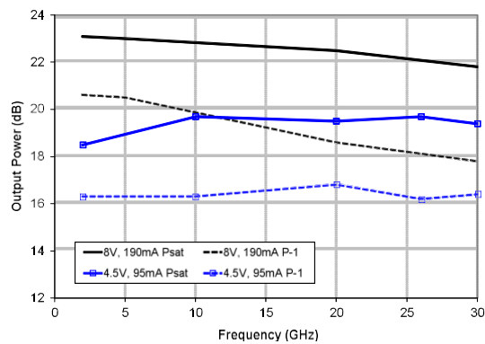
Output Power
