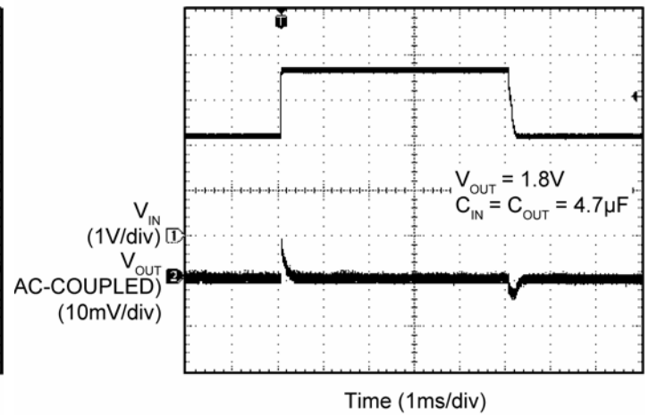
Line Transient
