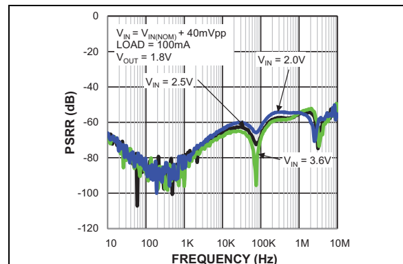
FIGURE 2-6: PSRR C_{OUT} = 2.2 \mu F .
