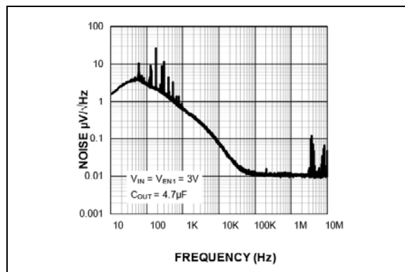
FIGURE 2-16: Output Noise Spectral Density.
