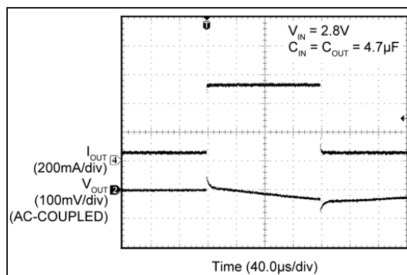
FIGURE 2-17: Load Transient.
