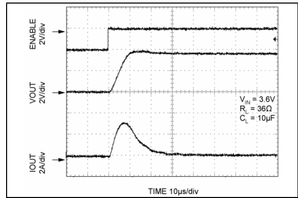
FIGURE 2-15: Turn-On/Turn-Off Timing.
