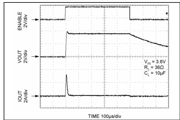
FIGURE 2-16: Turn-On/Turn-Off Timing.
