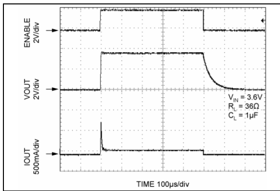
FIGURE 2-14: Turn-On/Turn-Off Timing.
