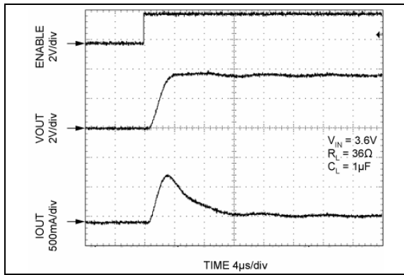
FIGURE 2-13: Turn-On/Turn-Off Timing.
