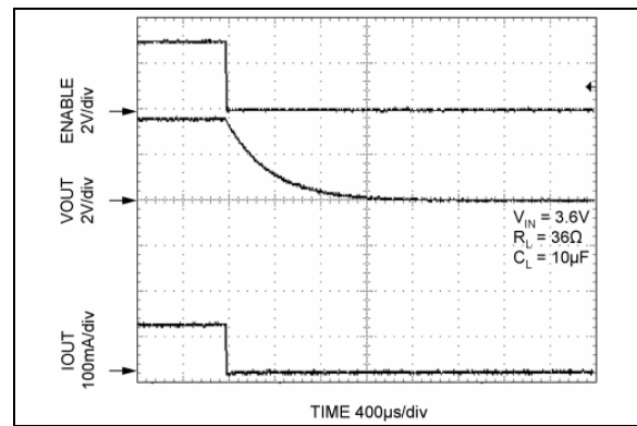
FIGURE 2-24: Turn-On/Turn-Off Timing.
