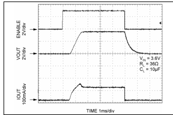
FIGURE 2-23: Turn-On/Turn-Off Timing.
