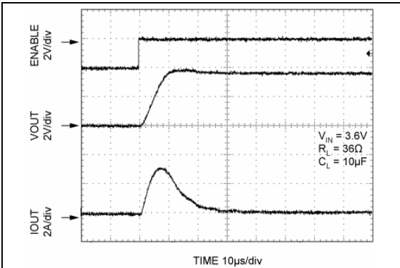
FIGURE 2-19: Turn-On/Turn-Off Timing.
