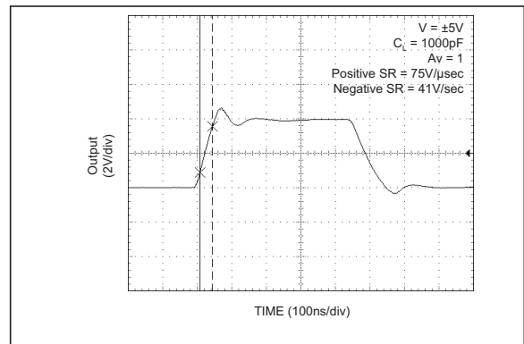
FIGURE 2-47: Large Signal Response.
