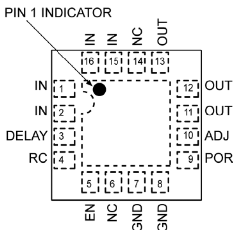
16-Pin 4mm × 4mm QFN
