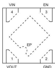
MIC5501/2/3/4 4-Lead UDFN (MT) (Top View)
