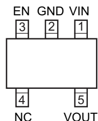
MIC5501/4 SOT23-5 (M5) (Top View)
