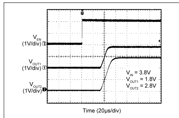
FIGURE 2-11: Turn-On Time.
