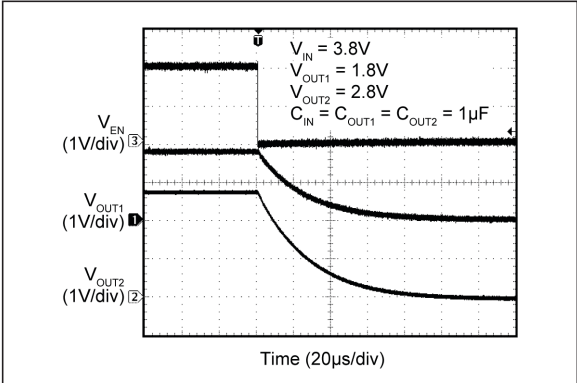
FIGURE 2-16: Turn-Off Time.
