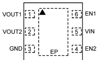
6-Pin 1.2mm x 1.2mm Thin DFN (MT) 6-Pin 1.2mm x 1.2mm Extra Thin DFN (MX) (Top View)
