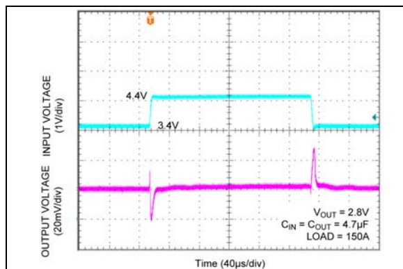
FIGURE 2-13: Line Transient 2.8V (3.4V to 4.4V).
