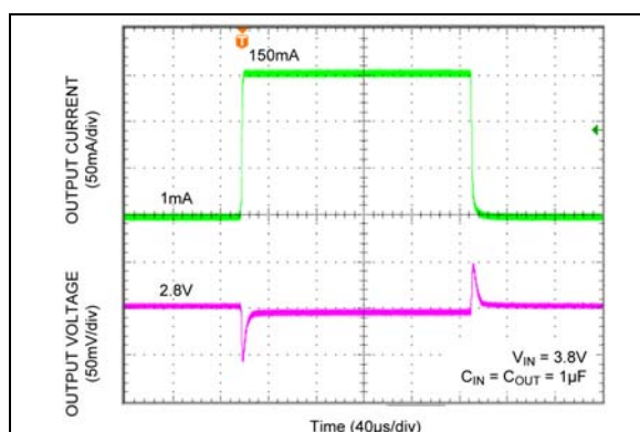
FIGURE 2-14: Load Transient 2.8V (1 mA to 150 mA).
