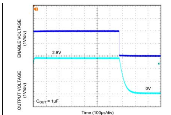
FIGURE 2-15: MIC5376 Auto-Discharge (No Load).
