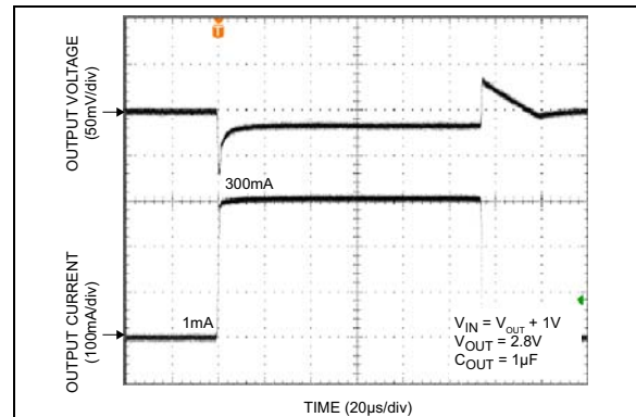
FIGURE 2-11: Load Transient.
