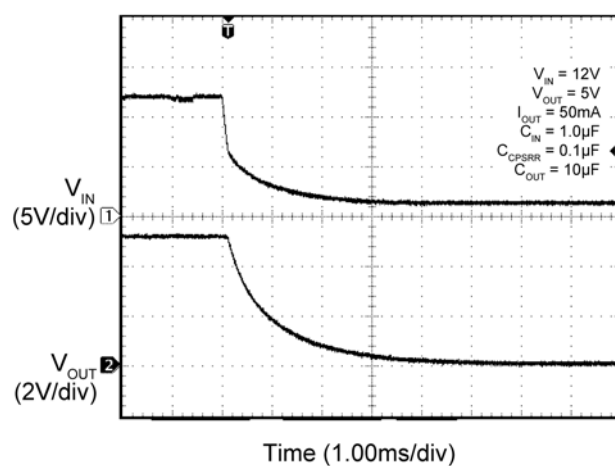
Fast Turn-Off
