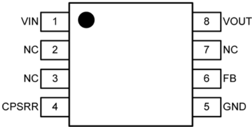
8-Pin MSOP MIC5281YMM (TOP VIEW)
