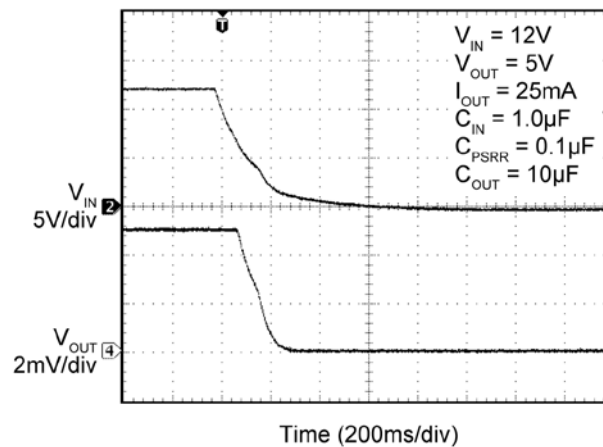
Soft Turn-Off
