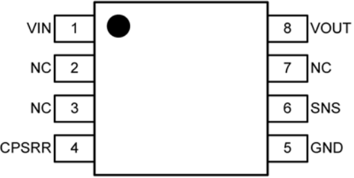
8-Pin MSOP MIC5281-x.xYMM (TOP VIEW)
