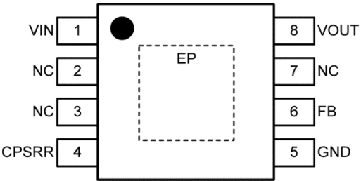
8-Pin ePAD MSOP MIC5281YMME (TOP VIEW)
