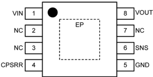
8-Pin ePAD MSOP MIC5281-x.xYMME (TOP VIEW)
