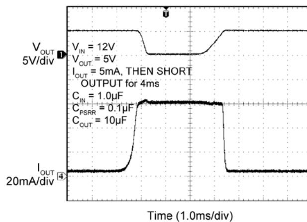
Current Limit
