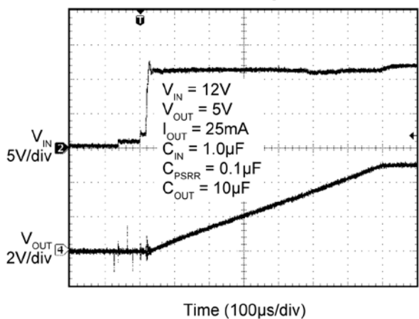
Hot Plug
