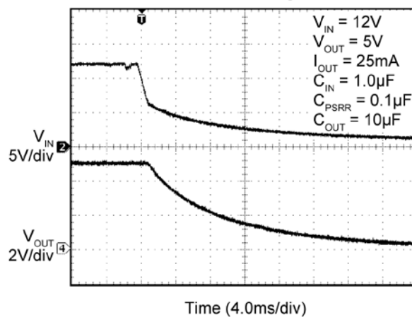
Hot Un-Plug
