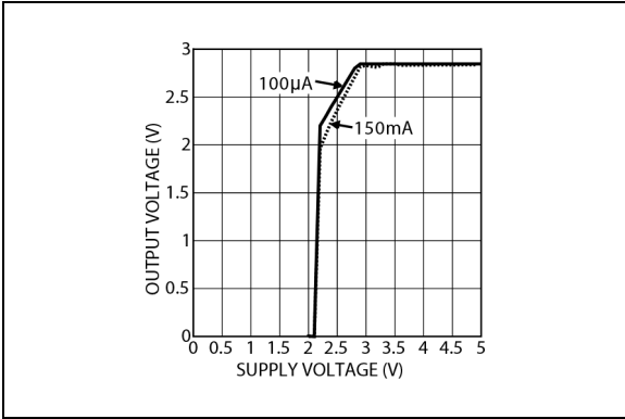
FIGURE 2-11: Dropout Characteristics.
