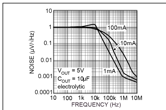
FIGURE 2-13: Noise Performance.
