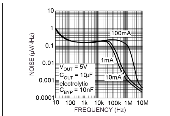
FIGURE 2-17: Noise Performance (Regulator B).
