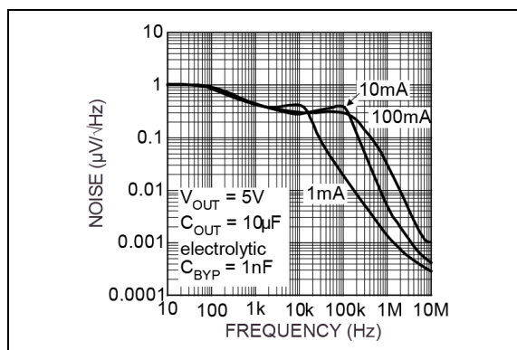
FIGURE 2-16: Noise Performance (Regulator B).
