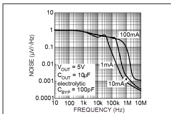
FIGURE 2-15: Noise Performance (Regulator B).
