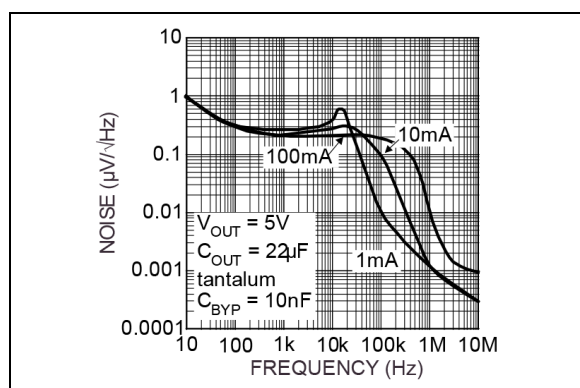
FIGURE 2-14: Noise Performance (Regulator B).
