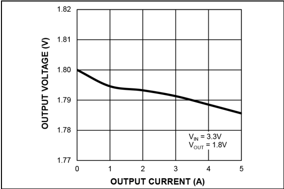
FIGURE 2-11: Output Voltage ( V_{IN} = 3.3V ) vs. Output Current.
