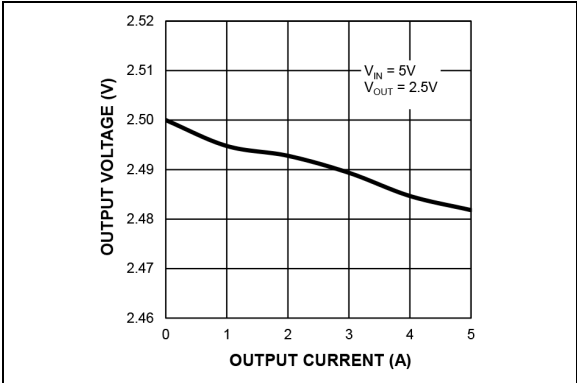
FIGURE 2-12: Output Voltage ( V_{IN} = 5V ) vs. Output Current.
