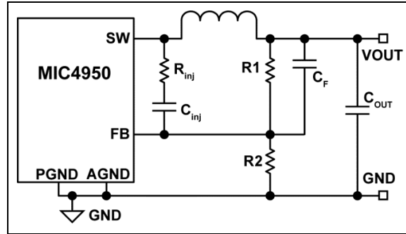
FIGURE 5-1: External Ripple Injection.
