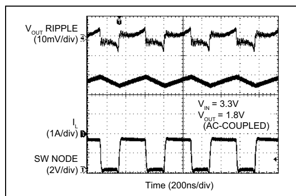
FIGURE 2-24: Switching Waveforms ( I_{OUT} = 2.5A ).
