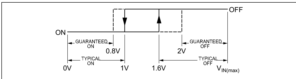
FIGURE 1-2: Shutdown Hysteresis.
