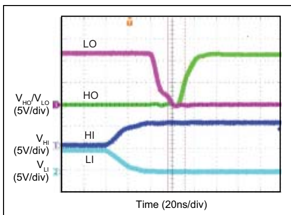
FIGURE 7-3: Adaptive Dead-Time LO (Low) to HO (High).
