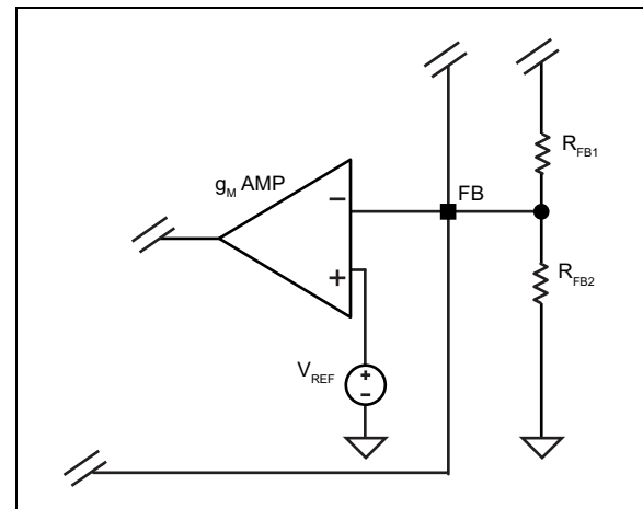
FIGURE 5-3: Voltage-Divider Configuration.
