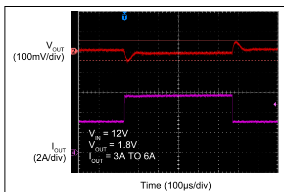
FIGURE 2-35: Load Transient Response, MIC45205-1 ( I_{OUT} = 3A to 6A ).
