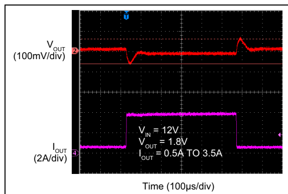
FIGURE 2-36: Load Transient Response, MIC45205-1 ( I_{OUT} = 0.5A to 3.5A ).
