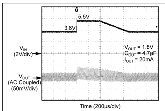
FIGURE 2-32: Line Transient (3.6V to 5.5V) at 20 mA.
