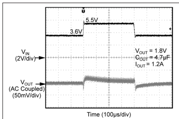
FIGURE 2-31: Line Transient (3.6V to 5.5V) at 1.2A.
