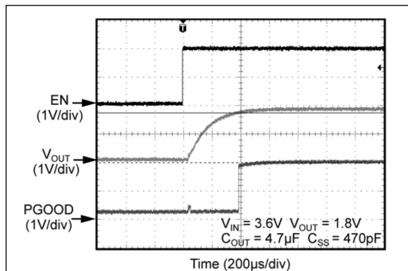
FIGURE 2-33: Start-Up with PGOOD ( C_{SS} = 470 pF ).
