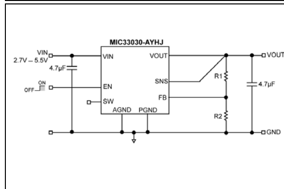
FIGURE 4-1: MIC33030-AYHJ Schematic.
