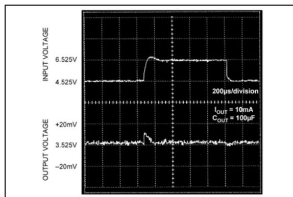
FIGURE 2-4: Line Transient Response with 100 mA Load, 100 μF Output Capacitance.
