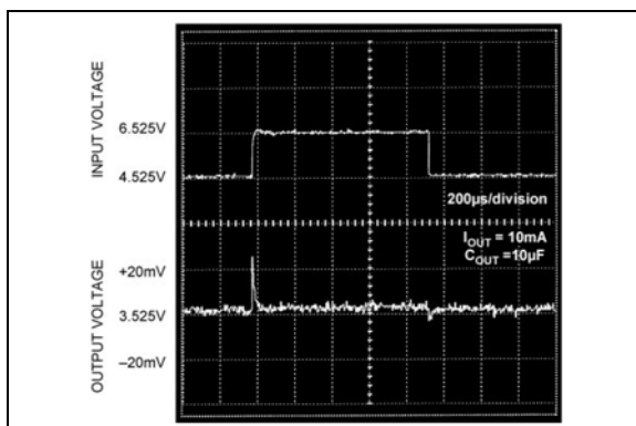
FIGURE 2-3: Line Transient Response with 10 mA Load, 10 μF Output Capacitance.
