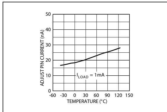
FIGURE 2-16: MIC29202 Adjust Pin Current vs. Temperature.
