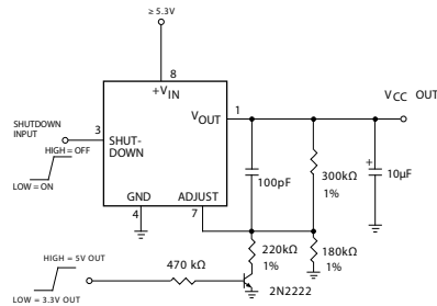
MIC29202/4 5V OR 3.3V SELECTABLE REGULATOR WITH SHUTDOWN (PINOUT FOR MIC29204)
