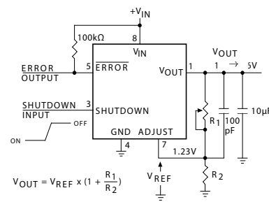
MIC29202/4 ADJUSTABLE REGULATOR (PINOUT FOR MIC29204)
