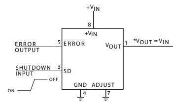
MIC29204 WIDE INPUT VOLTAGE RANGE CURRENT LIMITER
