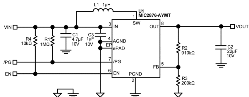
MIC2876-AYMT Typical Application Schematic – V_{IN} \leq 5.0V
