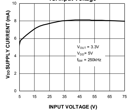
V_{DD} Operating Supply Current vs. Input Voltage
