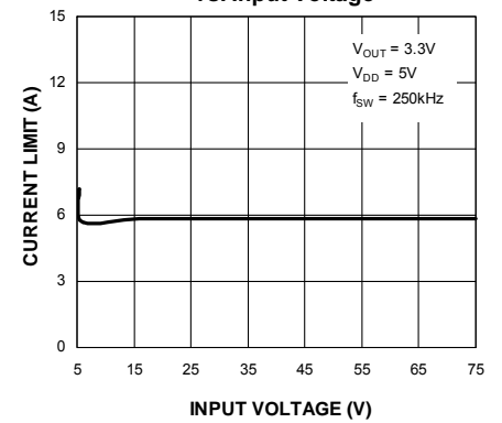
Output Peak Current Limit vs. Input Voltage
