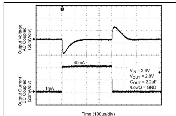
FIGURE 2-23: LDO2 (LOWQ Mode) Load Transient.
