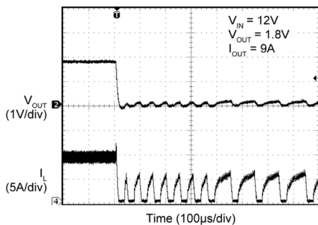
Short Circuit
