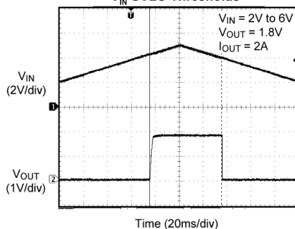
V_{IN} UVLO Thresholds
