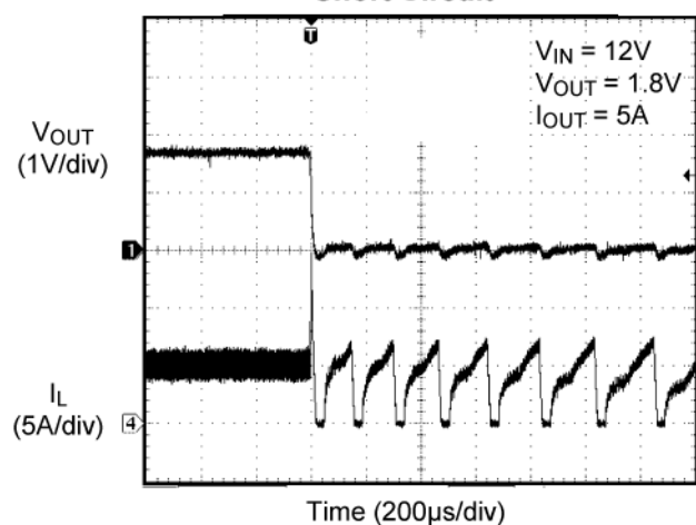
Short Circuit
