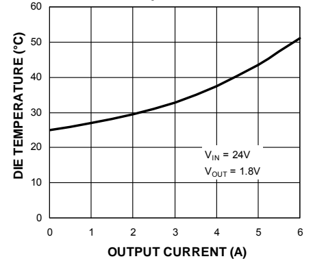
Die Temperature* ( V_{IN} = 24V ) vs. Output Current
