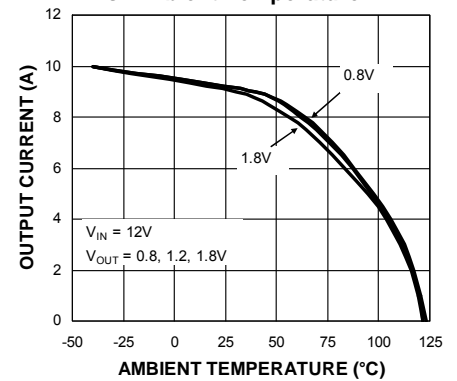
Thermal Derating* vs. Ambient Temperature
