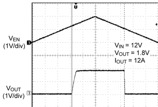
Enable Thresholds
