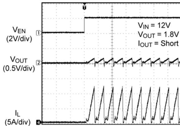
Enabled into Short
