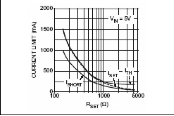
FIGURE 2-11: Current Limit vs. R_{SET} .
