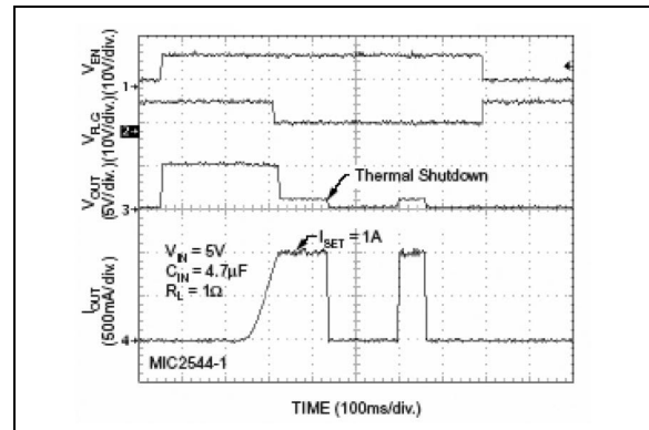
FIGURE 2-17: Current-Limit Response.
