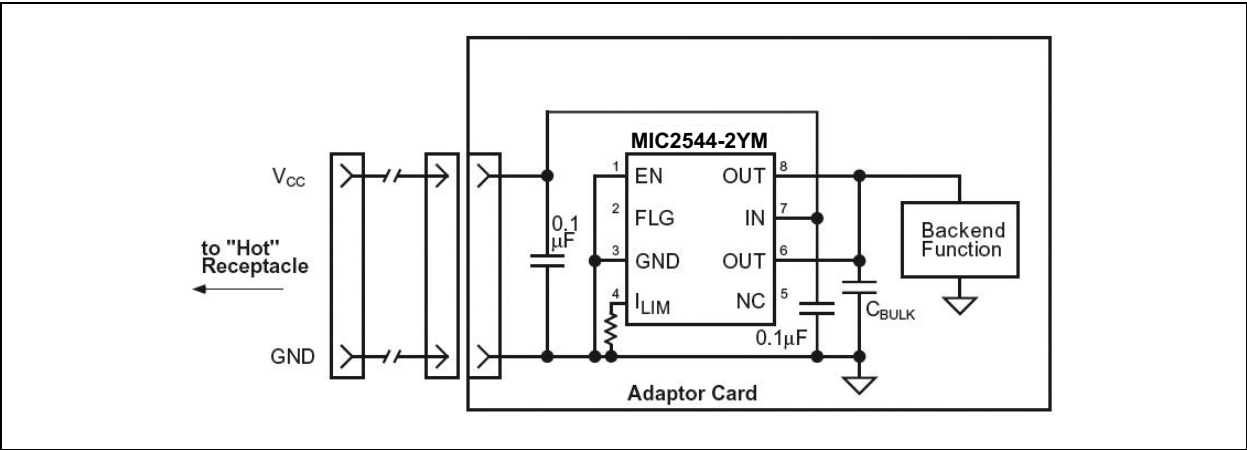
FIGURE 6-3: Hot Plug Application.
