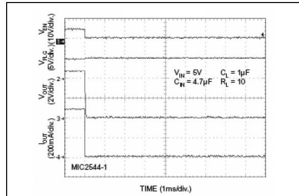
FIGURE 2-16: Turn-Off Response.
