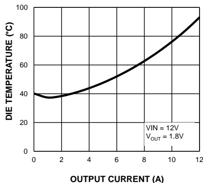
Die Temperature* (VIN = 12V) vs. Output Current
