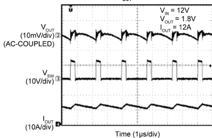
Switching Waveforms
