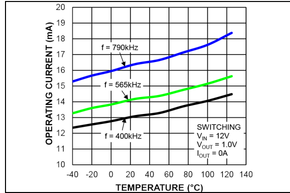
FIGURE 2-4: Operating Current ( I_Q ) vs. Temperature.
