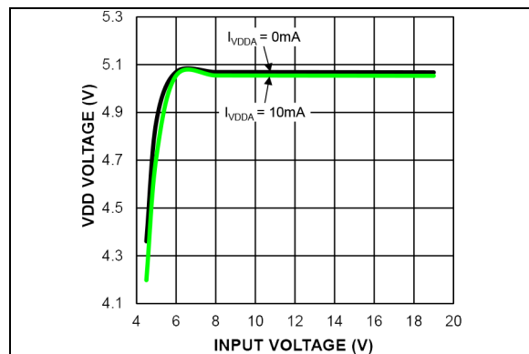
FIGURE 2-6: VDD Voltage vs. Input Voltage.
