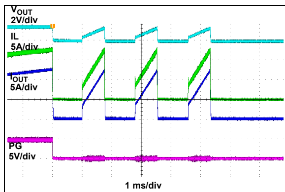
FIGURE 2-25: Output Current Limit Threshold.
