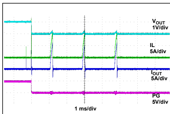
FIGURE 2-26: Hiccup Mode Short Circuit Current Limit Response.
