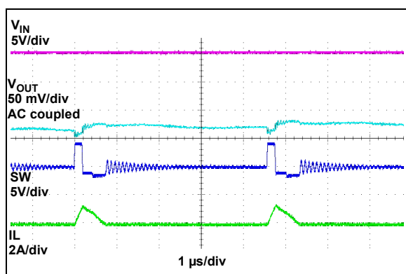
FIGURE 2-27: Switching Waveforms - I_{OUT} = 50mA , HLL.
