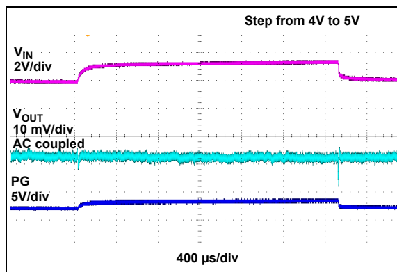
FIGURE 2-30: Line Transient Response.
