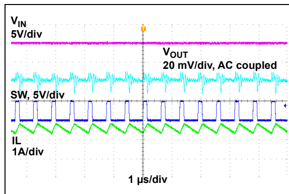
FIGURE 2-22: Switching Waveforms, I_{OUT} = 3A .
