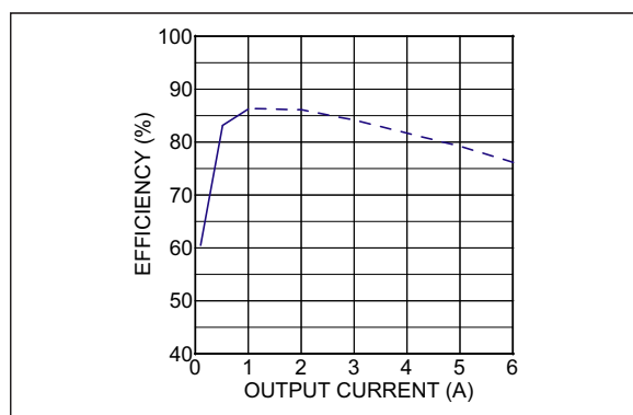
FIGURE 5-1: Efficiency 3.6V to 1.8V, L = 470 \text{ nH} .
