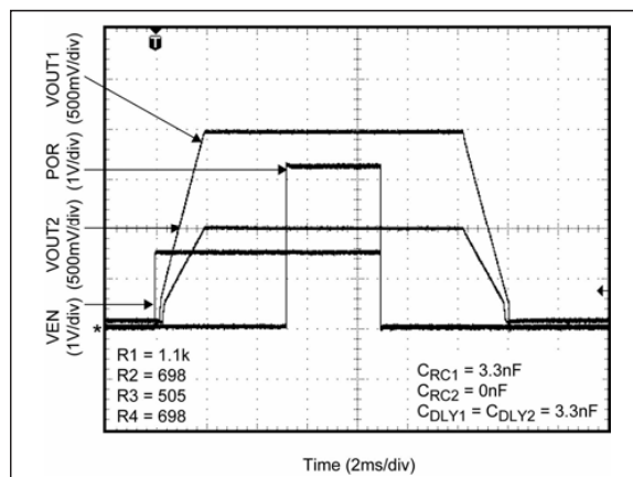
FIGURE 5-10: DDR Memory Tracking Example.
