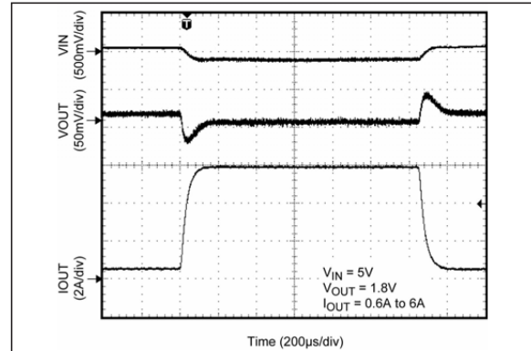
FIGURE 2-22: Transient Response.
