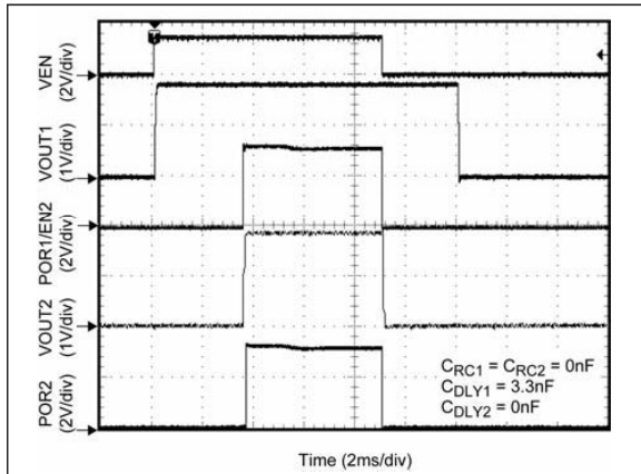
FIGURE 5-3: Window Sequencing Example.
