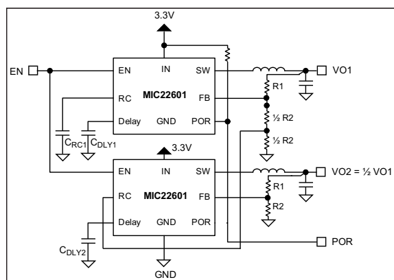
FIGURE 5-9: DDR Memory Tracking Circuit.
