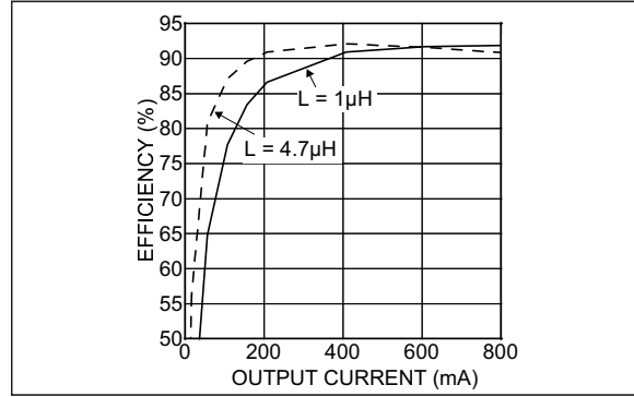
FIGURE 5-2: Efficiency vs. Inductance.
