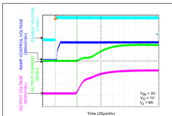
FIGURE 2-24: Start-Up ( C_{RC} = 0 \text{ nF} ).
