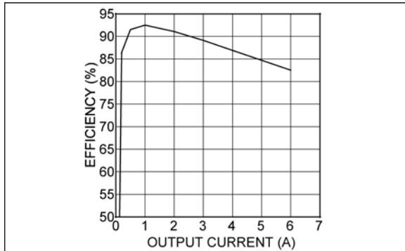
FIGURE 5-1: Efficiency Curve.
