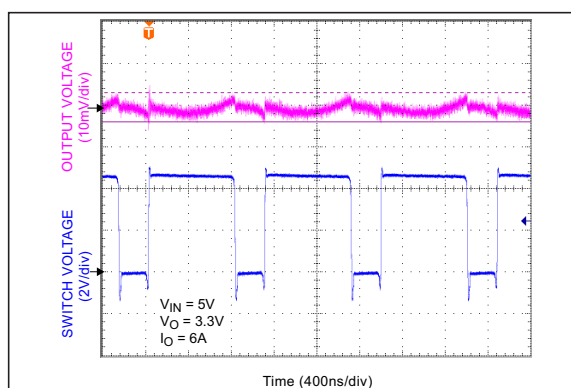
FIGURE 2-23: Output Noise and Ripple.
