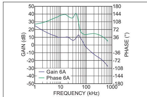
FIGURE 2-18: Bode Plot ( V_{IN} = 5.0V , V_O = 3.3V ).
