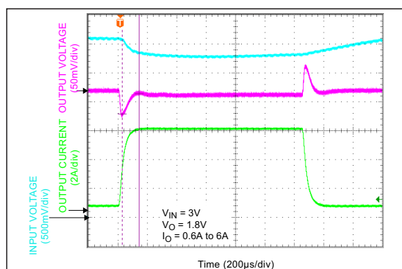
FIGURE 2-20: Transient Response.
