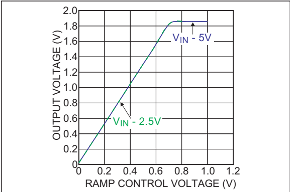
FIGURE 2-12: Output Voltage vs. Ramp Control Voltage.
