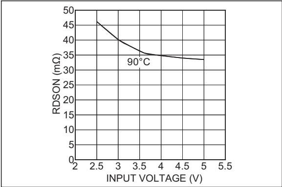
FIGURE 2-11: P-Channel R_{DS(ON)} vs. Input Voltage.
