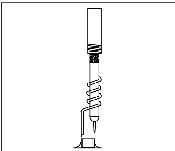
FIGURE 6-1: Ripple Measurement.
