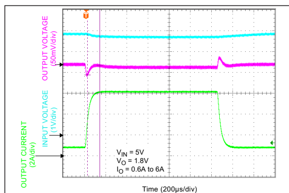
FIGURE 2-21: Transient Response.
