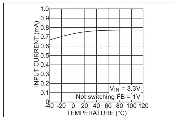
FIGURE 2-4: Operating Current vs. Temperature.
