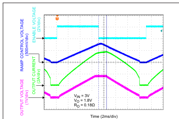
FIGURE 2-19: Start-Up/Shutdown ( C_{RC} = 10 \text{ nF} ).
