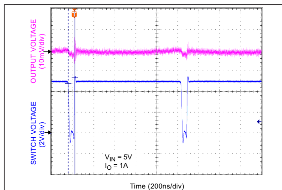
FIGURE 2-22: High DC Operation.
