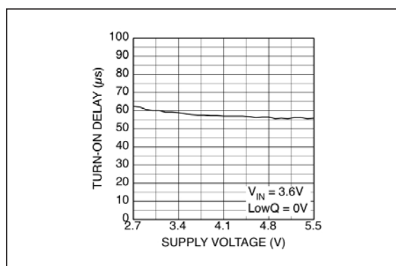
FIGURE 2-24: Turn-On Time vs. Supply Voltage.
