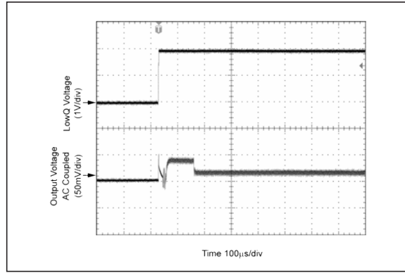
FIGURE 2-35: LDO Mode to PWM Mode Transient.
