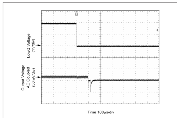
FIGURE 2-34: PWM Mode to LDO Mode Transient.
