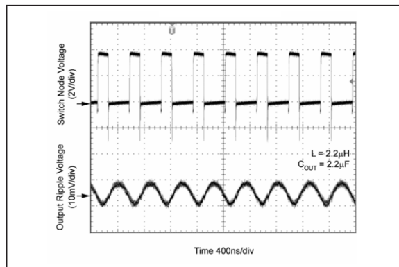
FIGURE 2-36: PWM Waveform.
