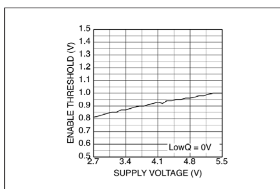
FIGURE 2-23: Enable Threshold Voltage vs. Supply Voltage.
