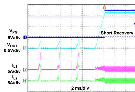
FIGURE 2-29: Output Short Recovery.
