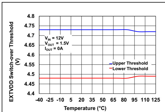
FIGURE 2-9: EXTVD Switchover Voltage vs. Temperature.
