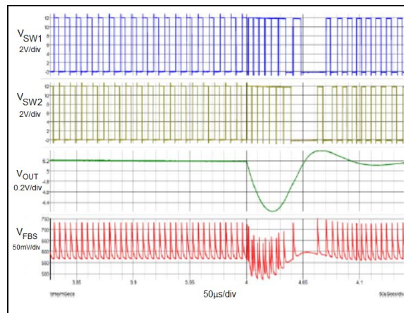
FIGURE 4-3: MIC21LV32 Load Transient Response.
