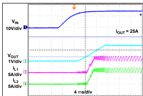
FIGURE 2-26: V_{IN} Power-up with 25A Load.
