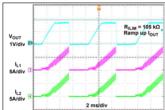
FIGURE 2-27: Current Limit per Phase.
