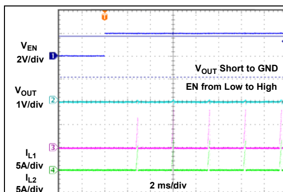
FIGURE 2-30: Enable into Short (EN from Low-to-High).
