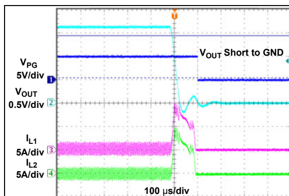
FIGURE 2-28: Output Short.
