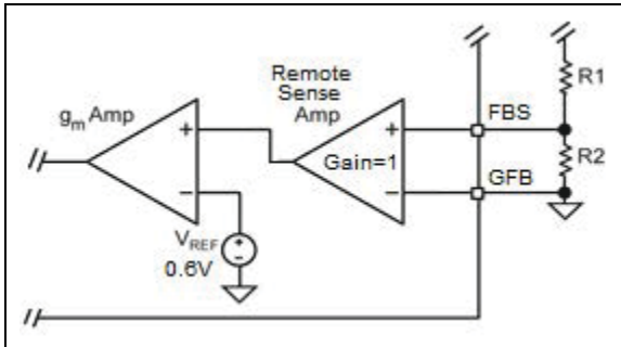
FIGURE 5-3: Voltage-Divider Configuration.
