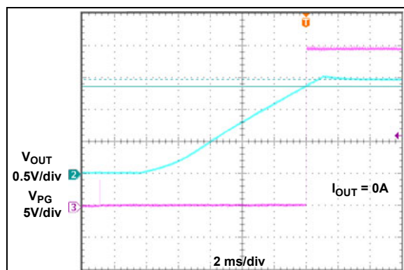
FIGURE 2-25: Power Good Response.
