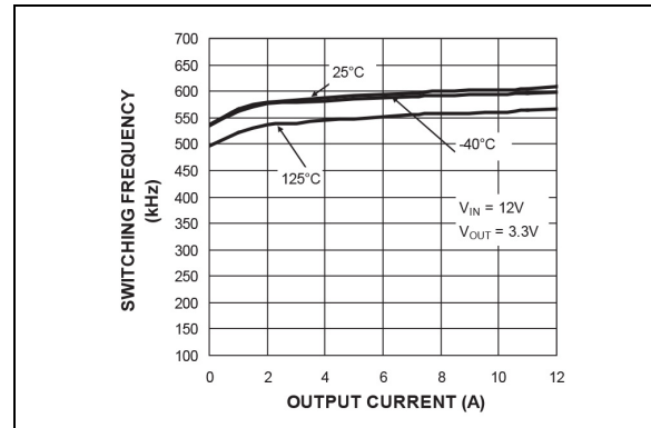
FIGURE 2-28: Switching Frequency vs. Output Current (MIC2102).
