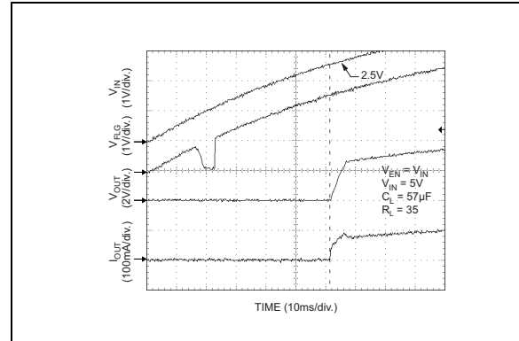
FIGURE 2-16: UVLO V_{IN} Rising (MIC2025-1).
