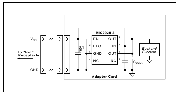
FIGURE 5-1: Hot-Plug Application.
