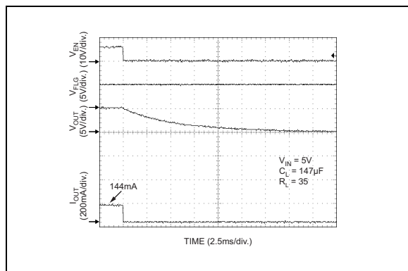
FIGURE 2-19: Turn-Off Response (MIC2025-1).
