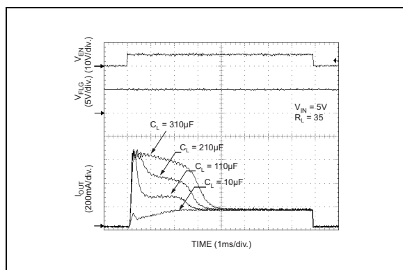
FIGURE 2-20: In-Rush Current Response (MIC2025-1).
