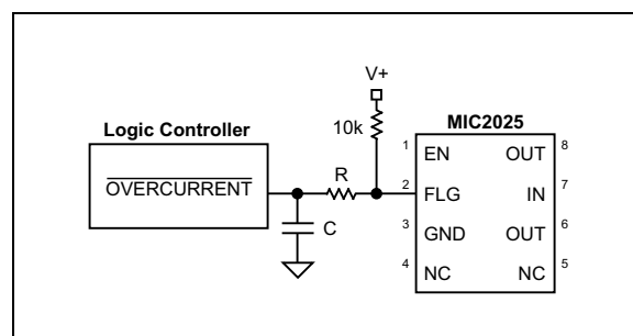
FIGURE 5-2: Transient Filter.
