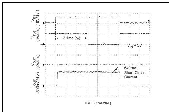
FIGURE 2-21: Enable Into Short (MIC2025-1).
