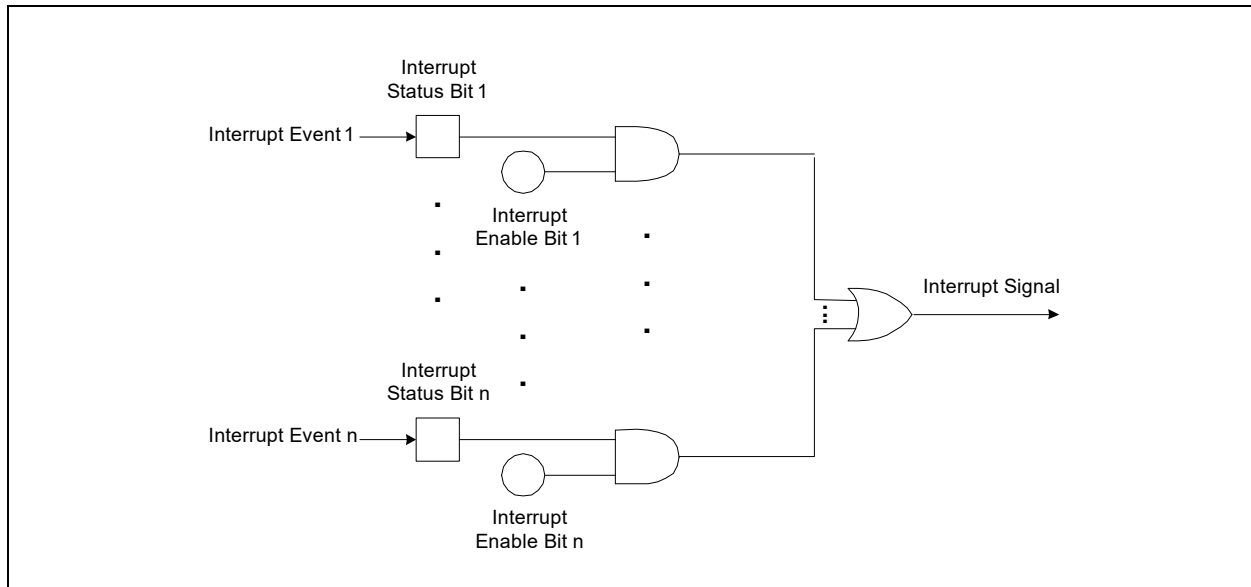
FIGURE 31-4: INTERRUPT FLOW
