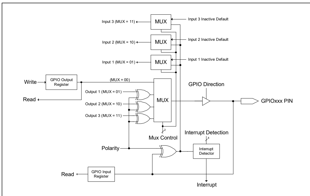
FIGURE 18-1: GPIO BLOCK DIAGRAM
