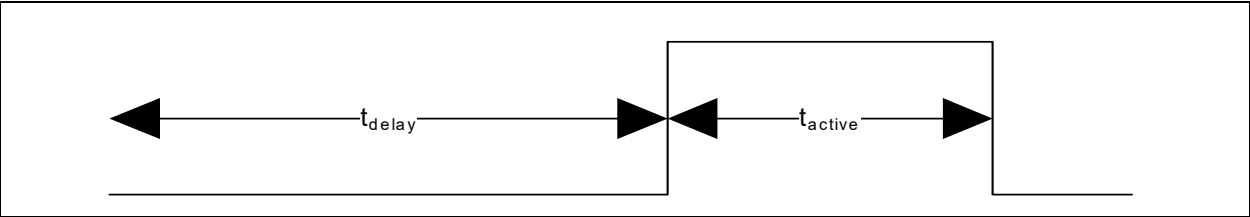
FIGURE 50-9: KBRST TIMING
