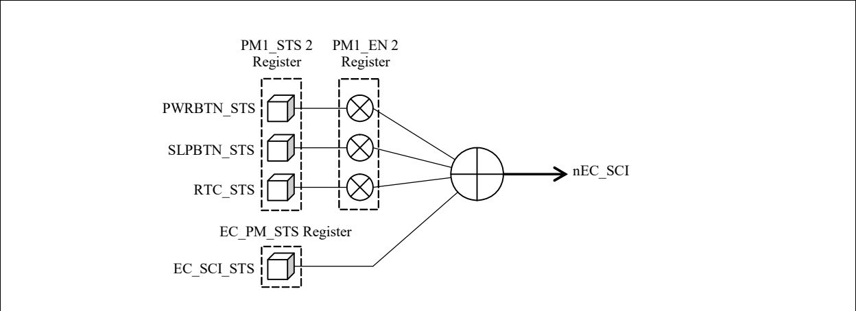
FIGURE 13-2: EC_SCI# INTERFACE
