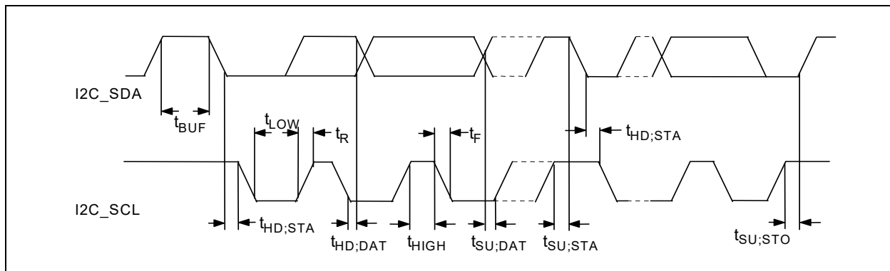
FIGURE 50-15: I2C/SMBUS TIMING
