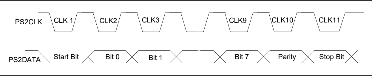
FIGURE 39-3: PS/2 PORT PHYSICAL LAYER BYTE TRANSMISSION PROTOCOL
