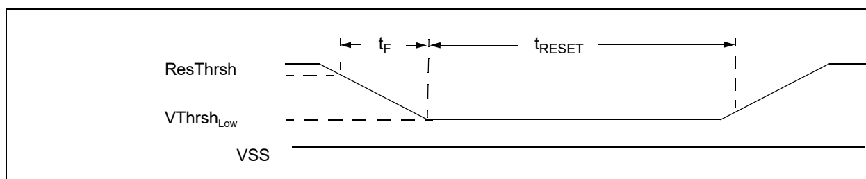
FIGURE 50-2: VTR RESET AND POWER-DOWN
