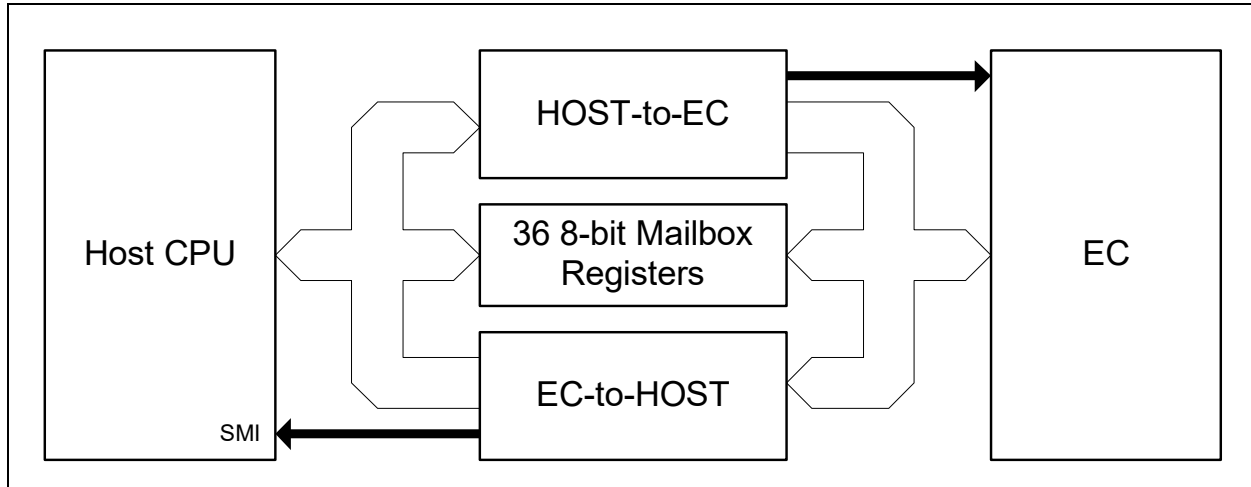
FIGURE 15-2: MAILBOX BLOCK DIAGRAM
