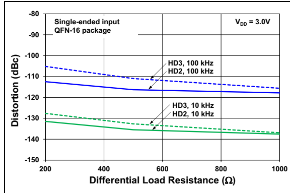
FIGURE 3-26: HD2, HD3 vs R_L , V_{OUTDM} = 2\text{Vpp} .
