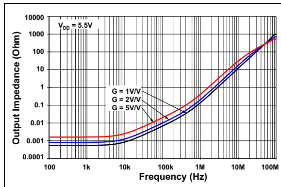
FIGURE 3-19: Closed-Loop, Differential Output Impedance vs. Frequency (Simulation).
