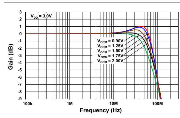
FIGURE 3-5: Small-Signal Frequency Response vs. V_{OCM} , Gain = 1\text{V/V} .
