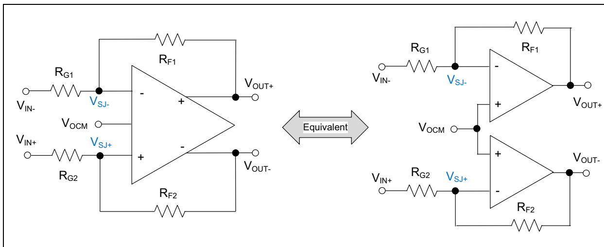
FIGURE 4-5: Equivalent Basic Circuit Functions.
