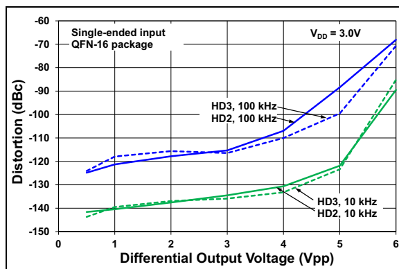
FIGURE 3-28: HD2, HD3 vs V_{OUTDM} , G = 1\text{V/V} .
