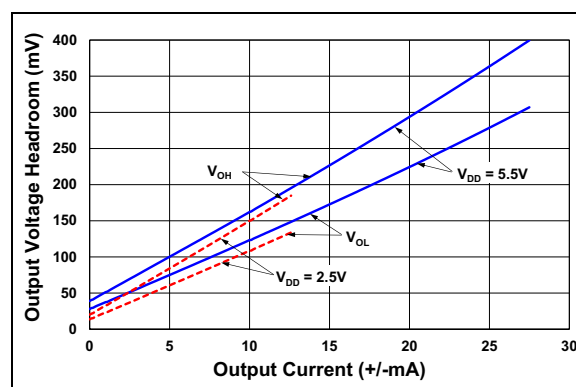
FIGURE 3-67: Output Voltage Headroom vs. Output Current.
