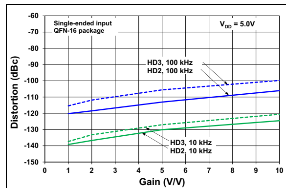
FIGURE 3-25: HD2, HD3 vs Gain, V_{OUTDM} = 2\text{Vpp} .
