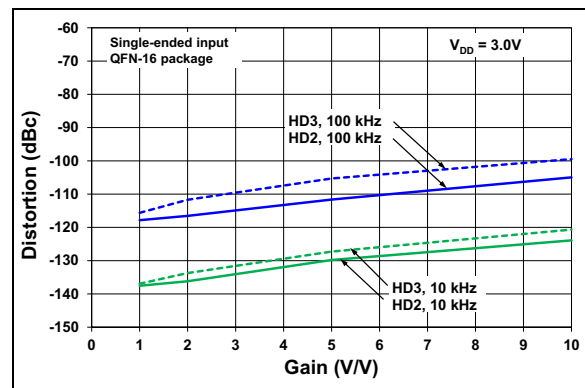
FIGURE 3-24: HD2, HD3 vs Gain, V_{OUTDM} = 2\text{Vpp} .
