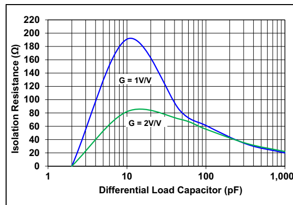
FIGURE 5-6: R_{ISO} vs. Differential Load Capacitor.
