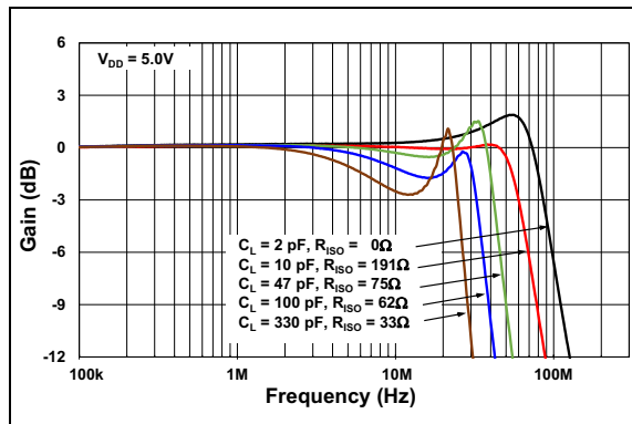
FIGURE 3-10: Small-Signal Frequency Response vs. C -Loads.
