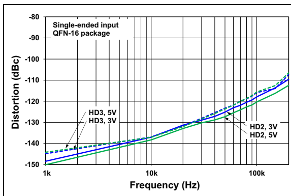
FIGURE 3-22: HD2, HD3 vs Frequency, V_{OUTDM} = 2\text{Vpp} .
