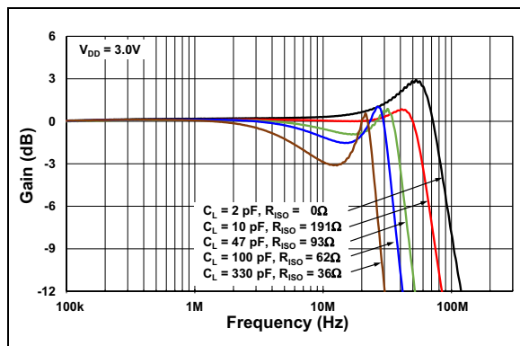
FIGURE 3-9: Small-Signal Frequency Response vs. C -Loads.
