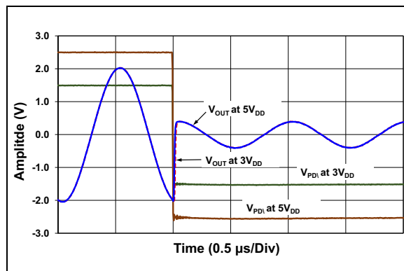
FIGURE 3-47: PDI Turn-Off Transient Response, Input Signal: 1\text{ MHz} Sine, 2\text{Vpp} .
