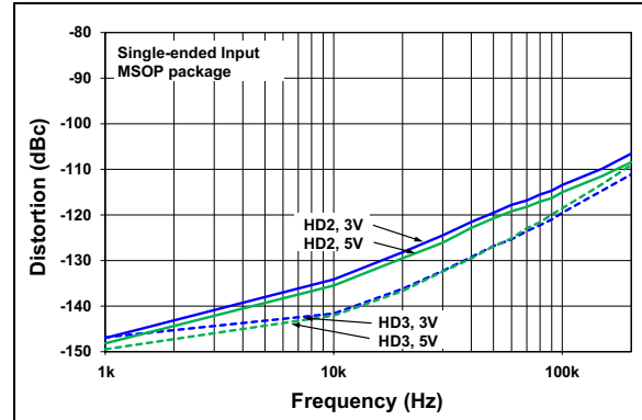
FIGURE 3-23: HD2 and HD3 vs. Frequency, V_{OUTDM} = 2\text{Vpp} .
