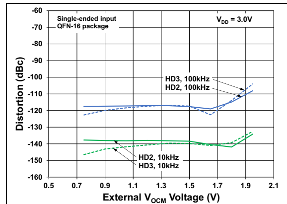
FIGURE 3-30: HD2, HD3 vs V_{OCM} , V_{OUTDM} = 2\text{Vpp} , Gain = 1\text{V/V} .
