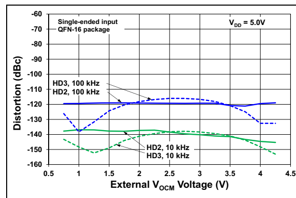
FIGURE 3-31: HD2, HD3 vs V_{OCM} , V_{OUTDM} = 2\text{Vpp} , Gain = 1\text{V/V} .
