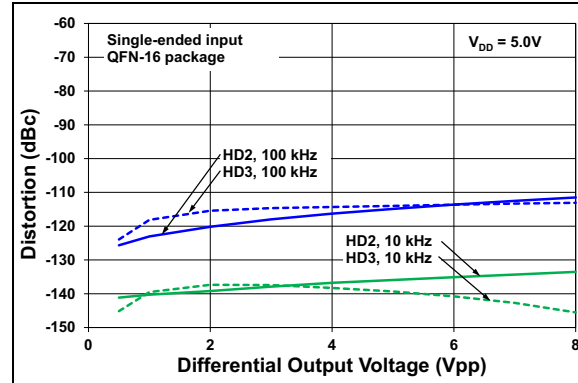
FIGURE 3-29: HD2, HD3 vs V_{OUTDM} , G = 1\text{V/V} .
