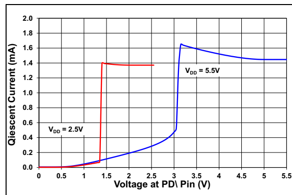
FIGURE 3-66: Supply Current vs. PD\ Voltage.
