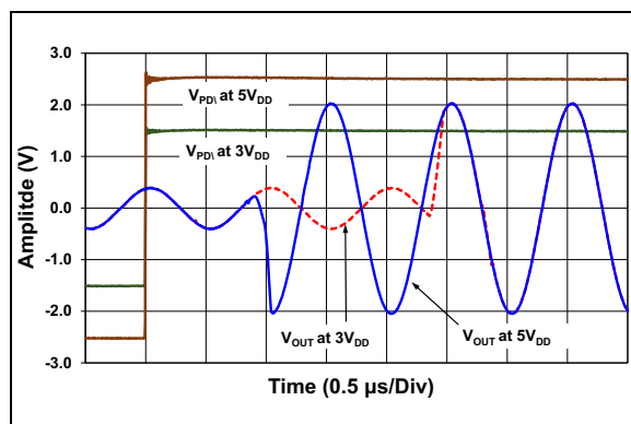
FIGURE 3-46: PDI Turn-On Transient Response, Input Signal: 1\text{ MHz} Sine, 2\text{Vpp} .
