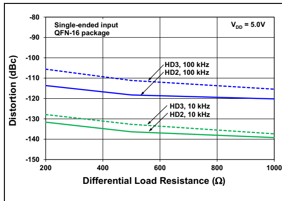
FIGURE 3-27: HD2, HD3 vs R_L , V_{OUTDM} = 2\text{Vpp} .
