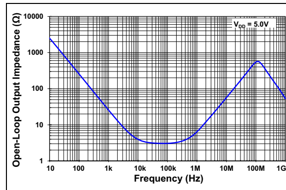
FIGURE 4-4: Simulated Open-Loop Differential Output Impedance.
