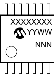
14-Lead TSSOP (MCP6034)
